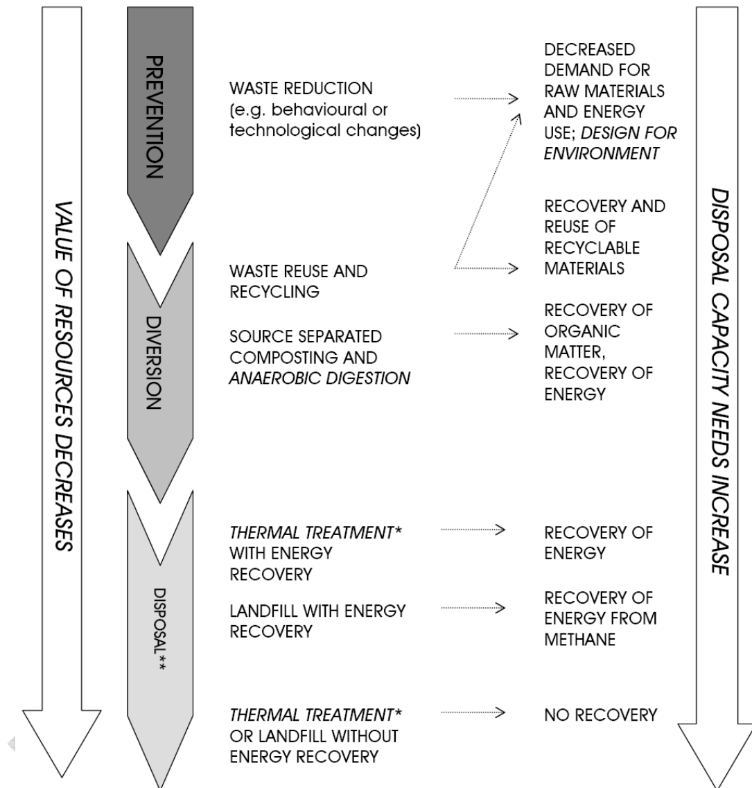
Figure 1.3: The Waste Value Chain or 'Lansink's Ladder' 4
