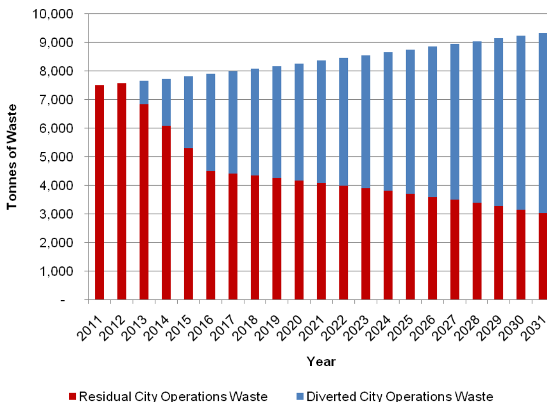
Figure 3.5: Estimated City Operations Residual Waste Disposed and Waste Diverted Year-by-Year over the Planning Period (2011-2031)
