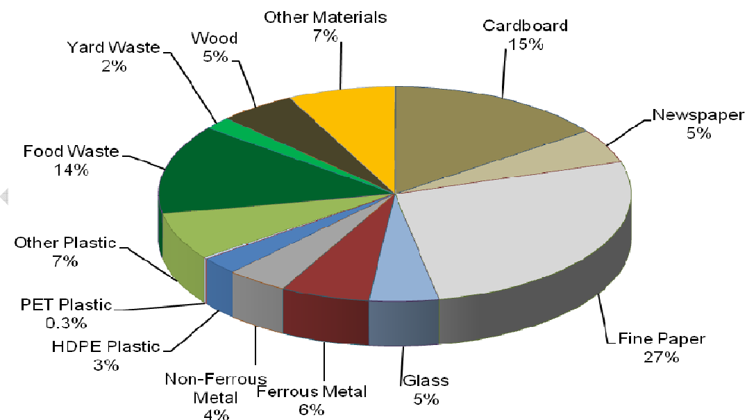
Figure 1.10: Estimated Composition of IC&amp;I Garbage Disposed at the Brady Road Landfill
