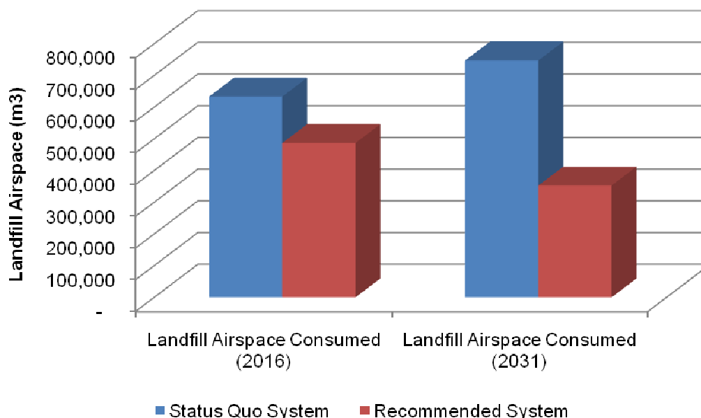
Figure 3.6: Comparison of Estimated Landfill Airspace Consumed at Brady Road under Status Quo and Recommended Waste Management Systems
