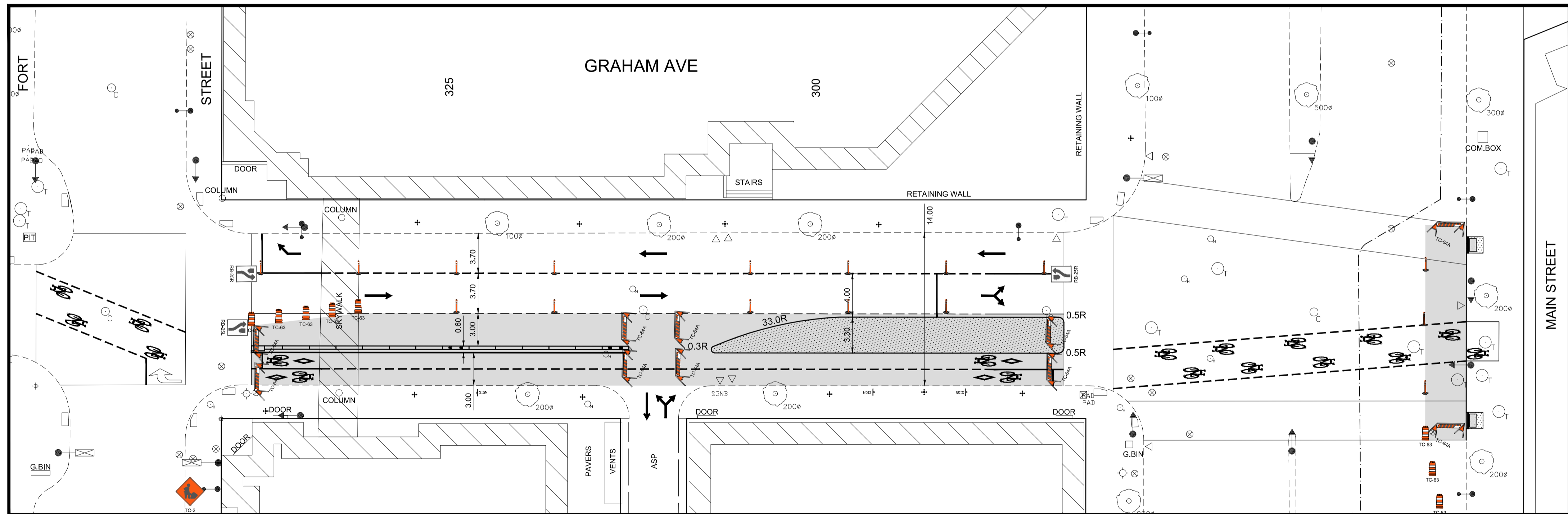
GRAHAM AVENUE - FORT STREET TO MAIN STREET - PLAN VIEW Scale 1:250
