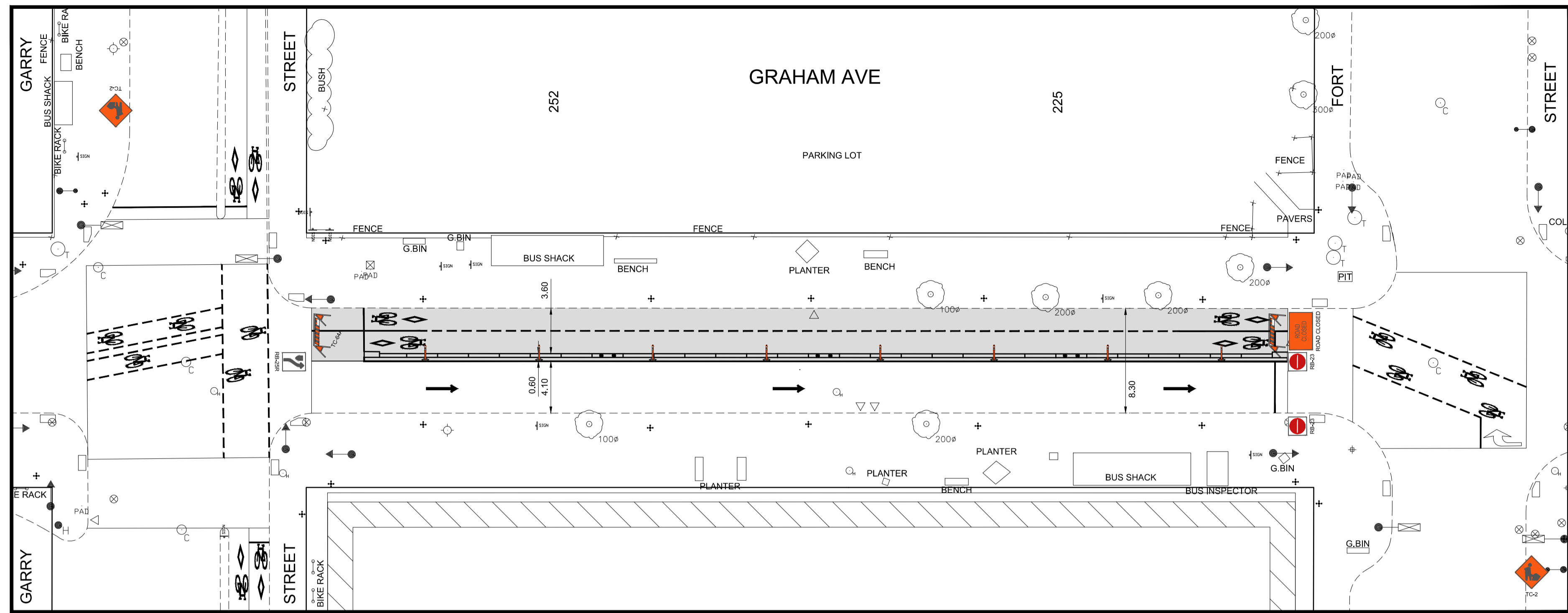
GRAHAM AVENUE - GARRY STREET TO FORT STREET - PLAN VIEW Scale 1:250
