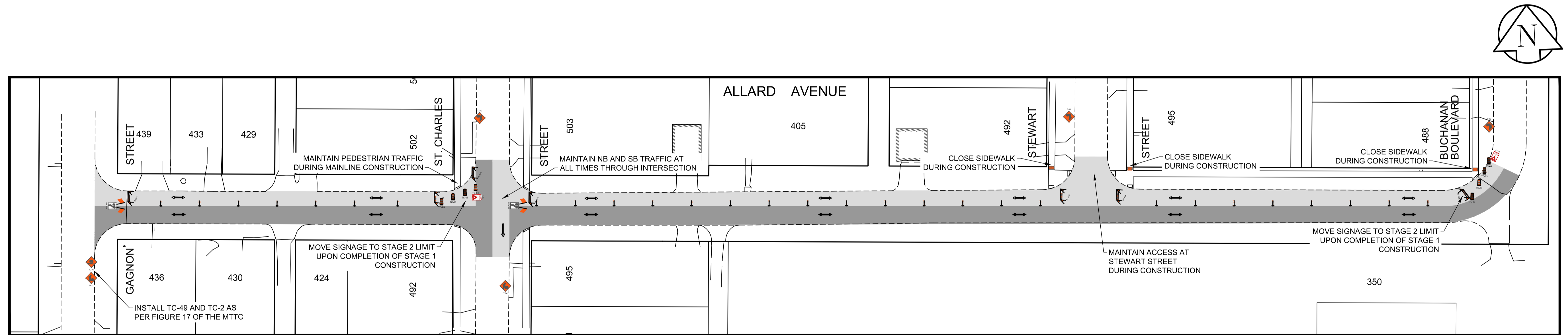
ALLARD AVENUE - GAGNON STREET TO BUCHANAN BOULEVARD - PLAN VIEW
