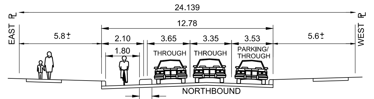
CROSS-SECTION STATION 1+320 NTS
