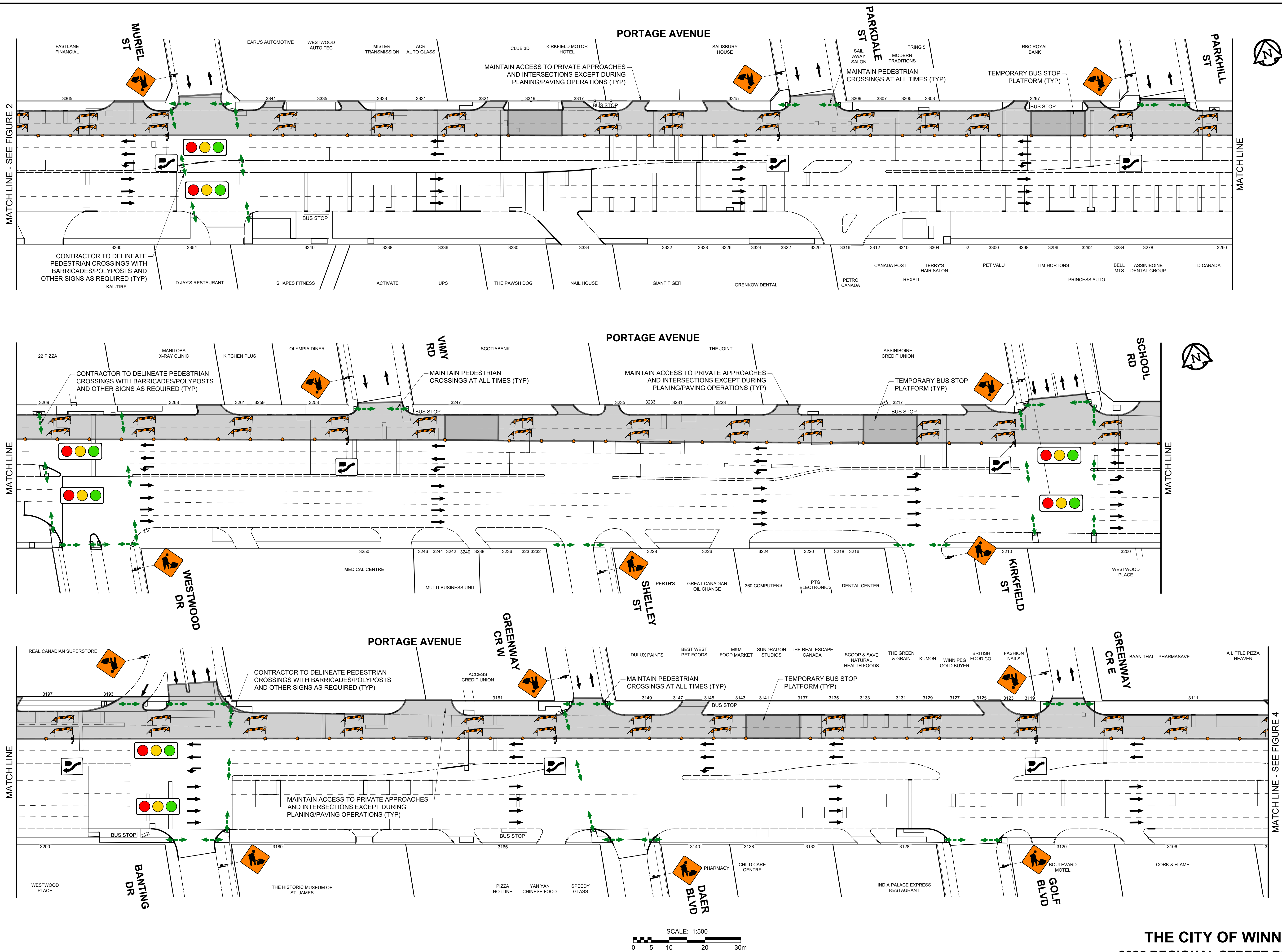
STAGE 1 WESTBOUND GUTTER LANES (2 OF 5) FIGURE 3
