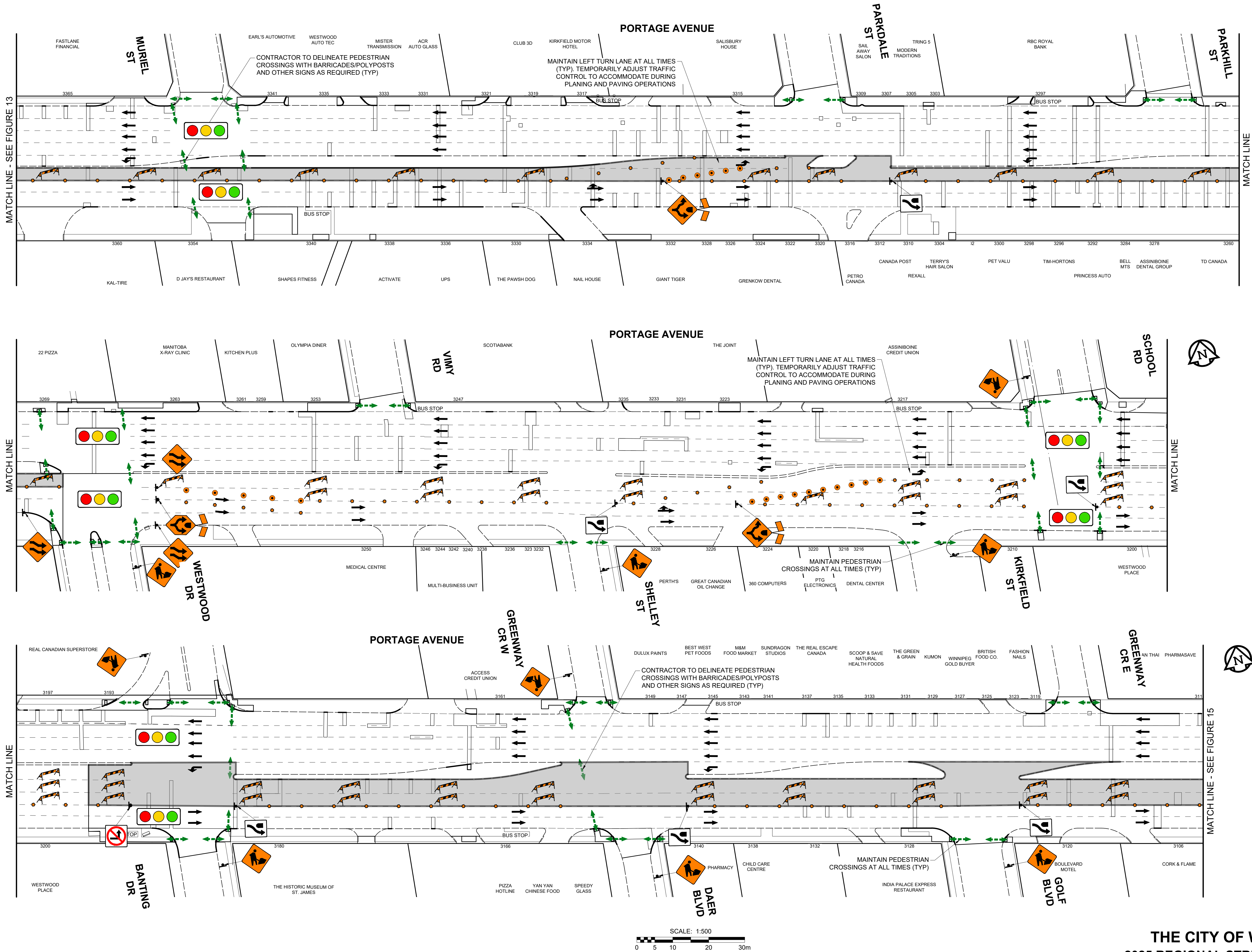
STAGE 5 EASTBOUND MEDIAN LANE (2 OF 4) FIGURE 16
