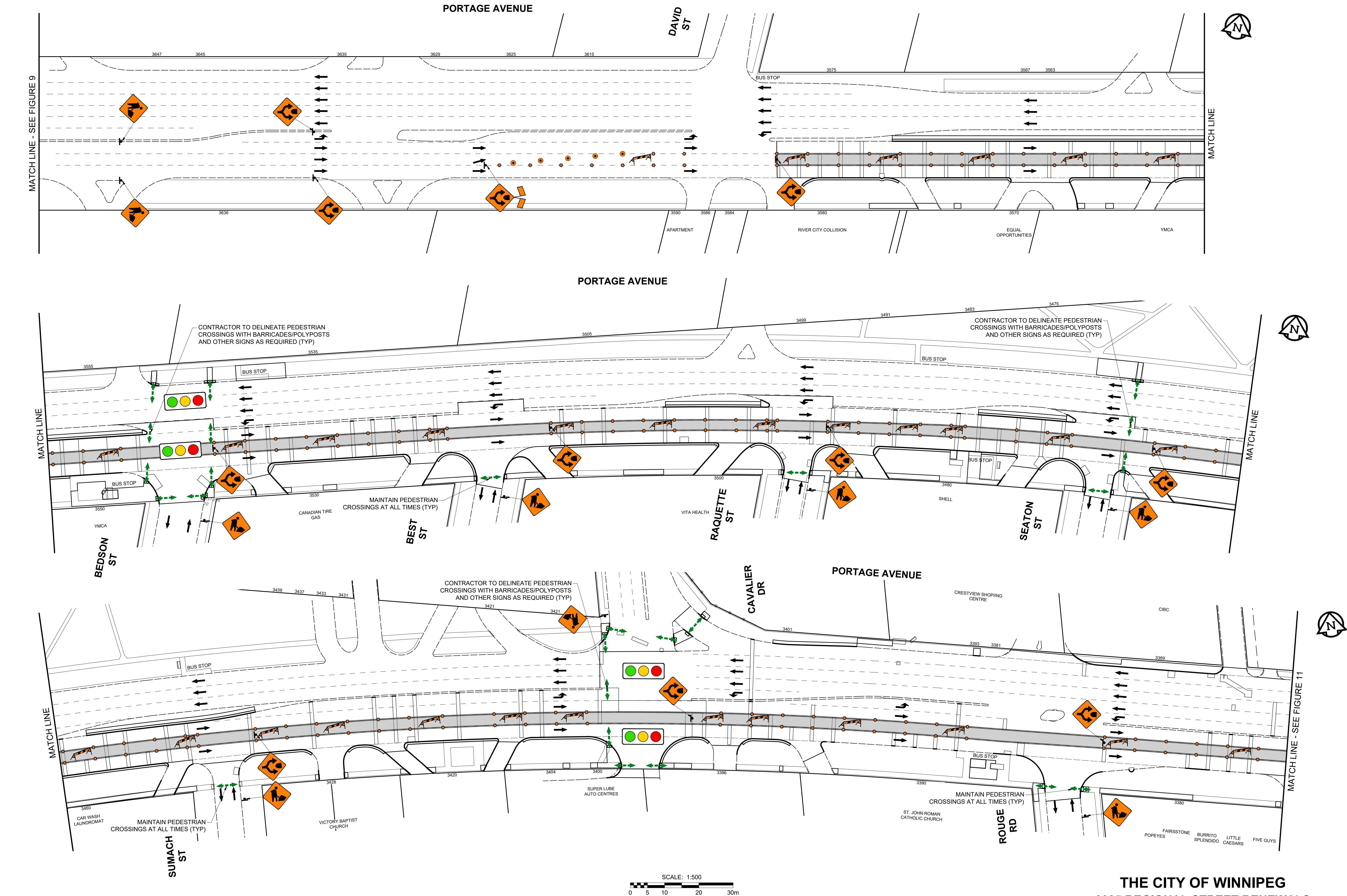
STAGE 4 EASTBOUND MIDDLE LANE (1 OF 3) FIGURE 12
