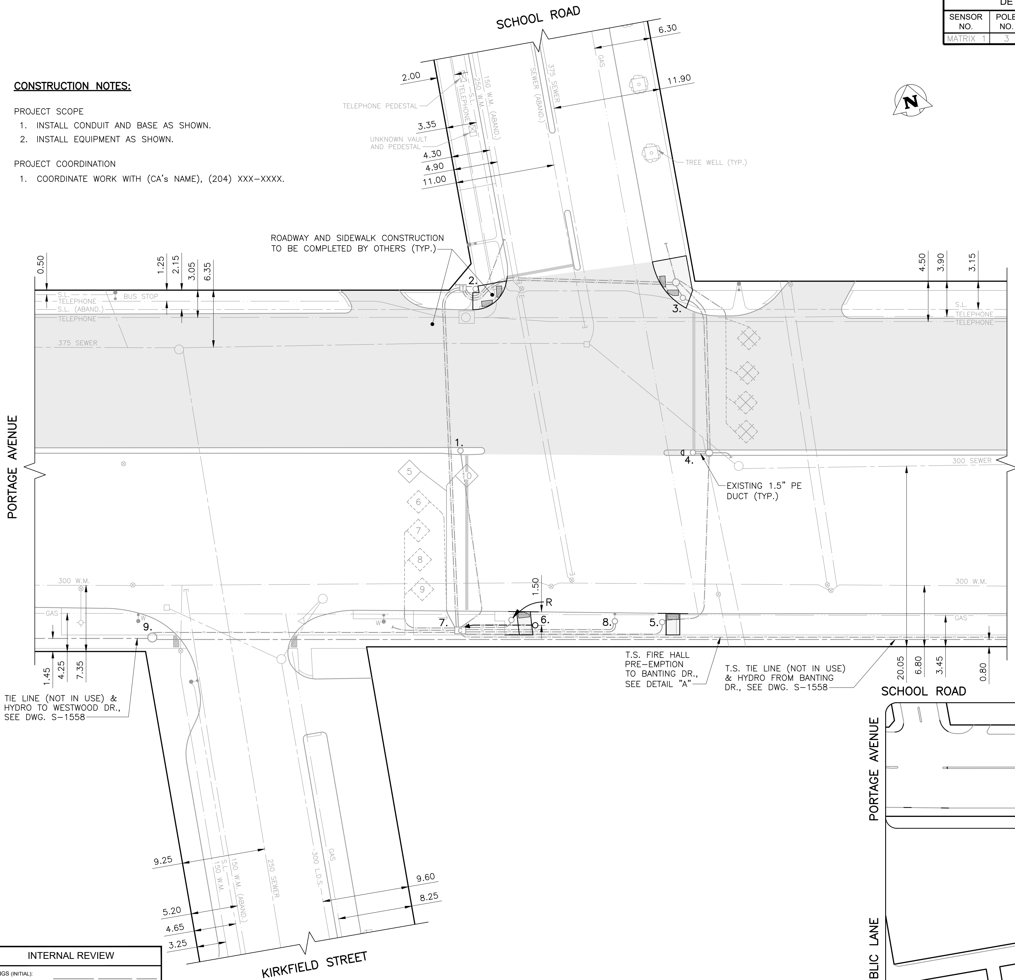
PLAN VIEW: UNDERGROUND CONSTRUCTION 1:250
