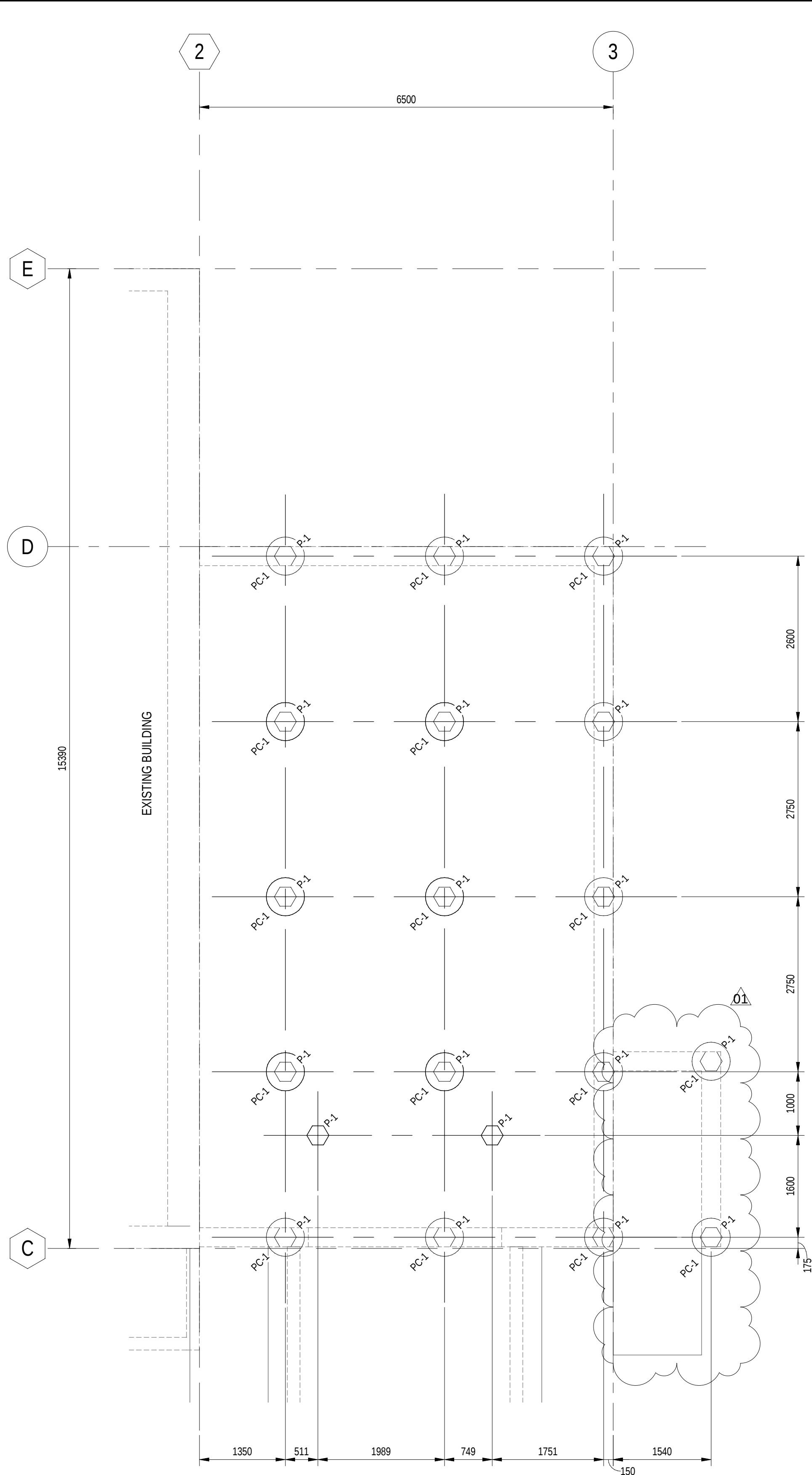
PLAN AT EL 231.278m SCALE: 1 : 50
