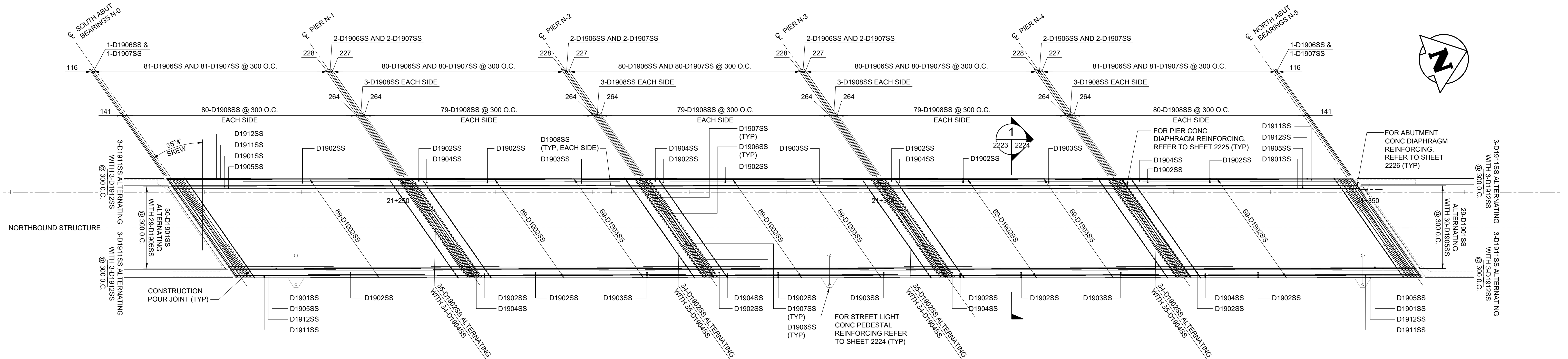
2 DECK REINF LAYOUT - TOP MAT 1 : 200
