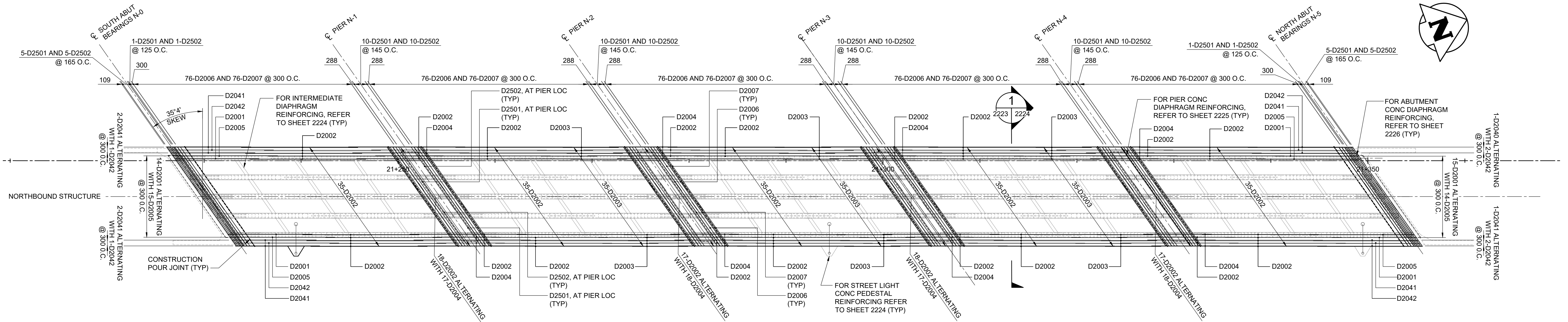
1 DECK REINF LAYOUT - BOTTOM MAT 1 : 200
