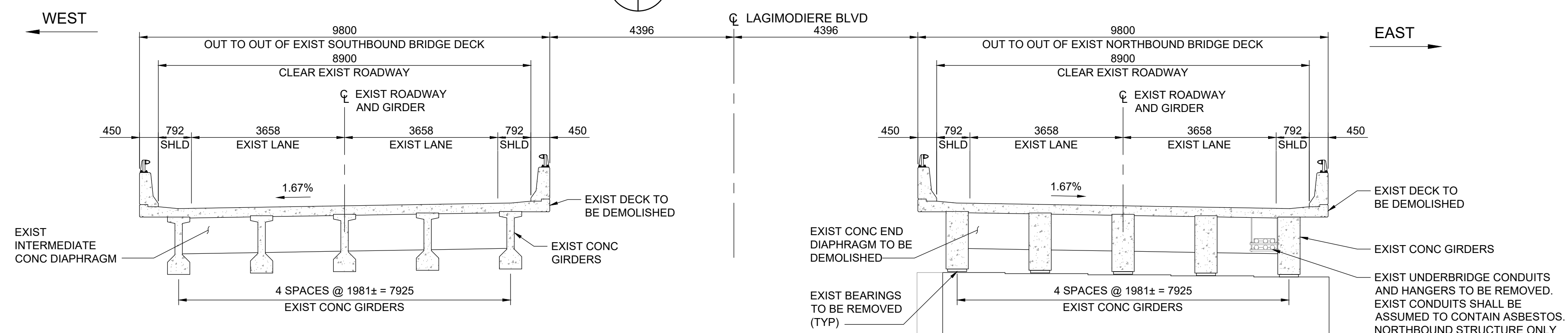
TYPICAL CROSS SECTION
