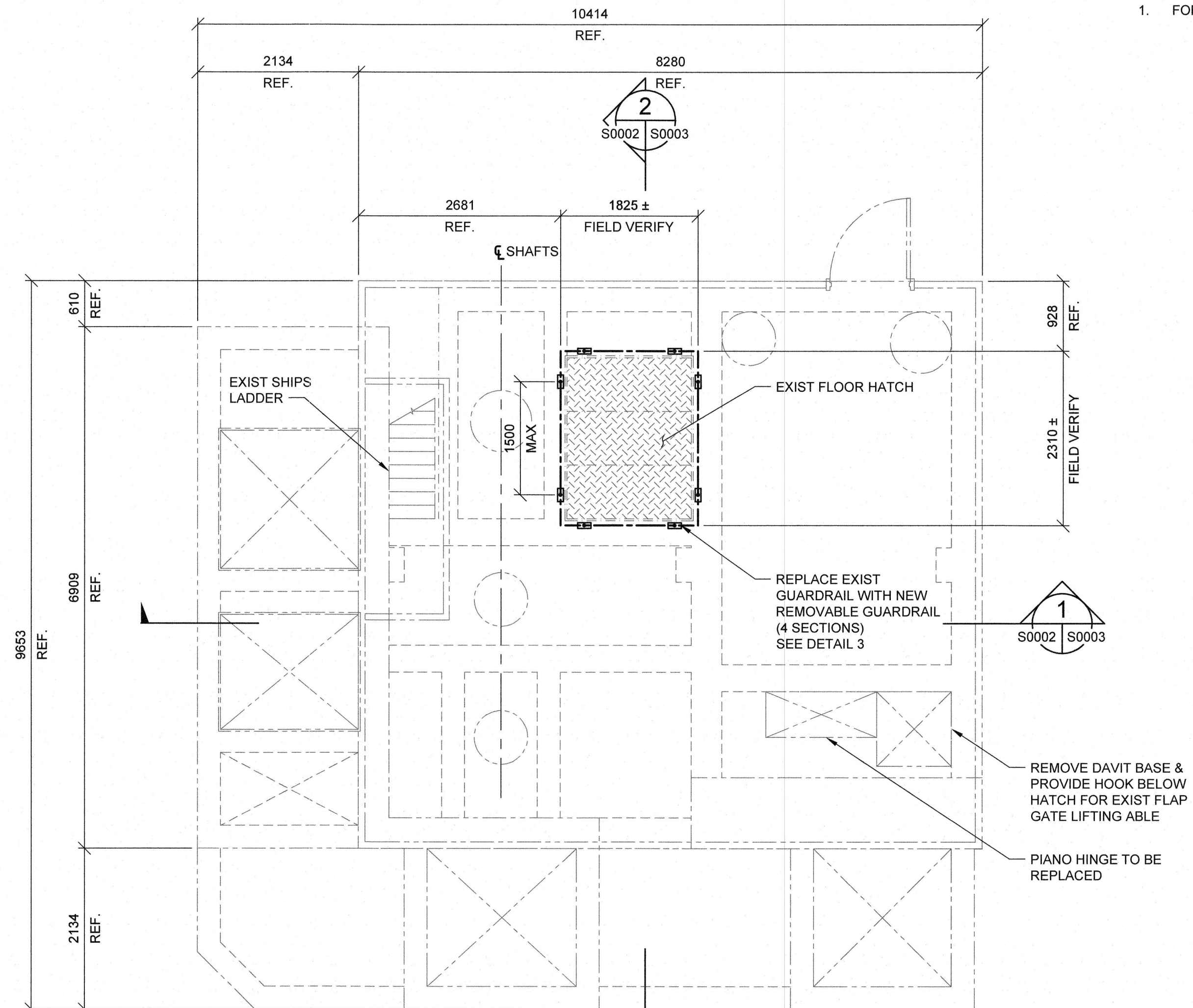
2 - - MOTOR FLOOR PLAN 1 : 50 T.O. EXIST MOTOR FLOOR @ EL. 231.587
