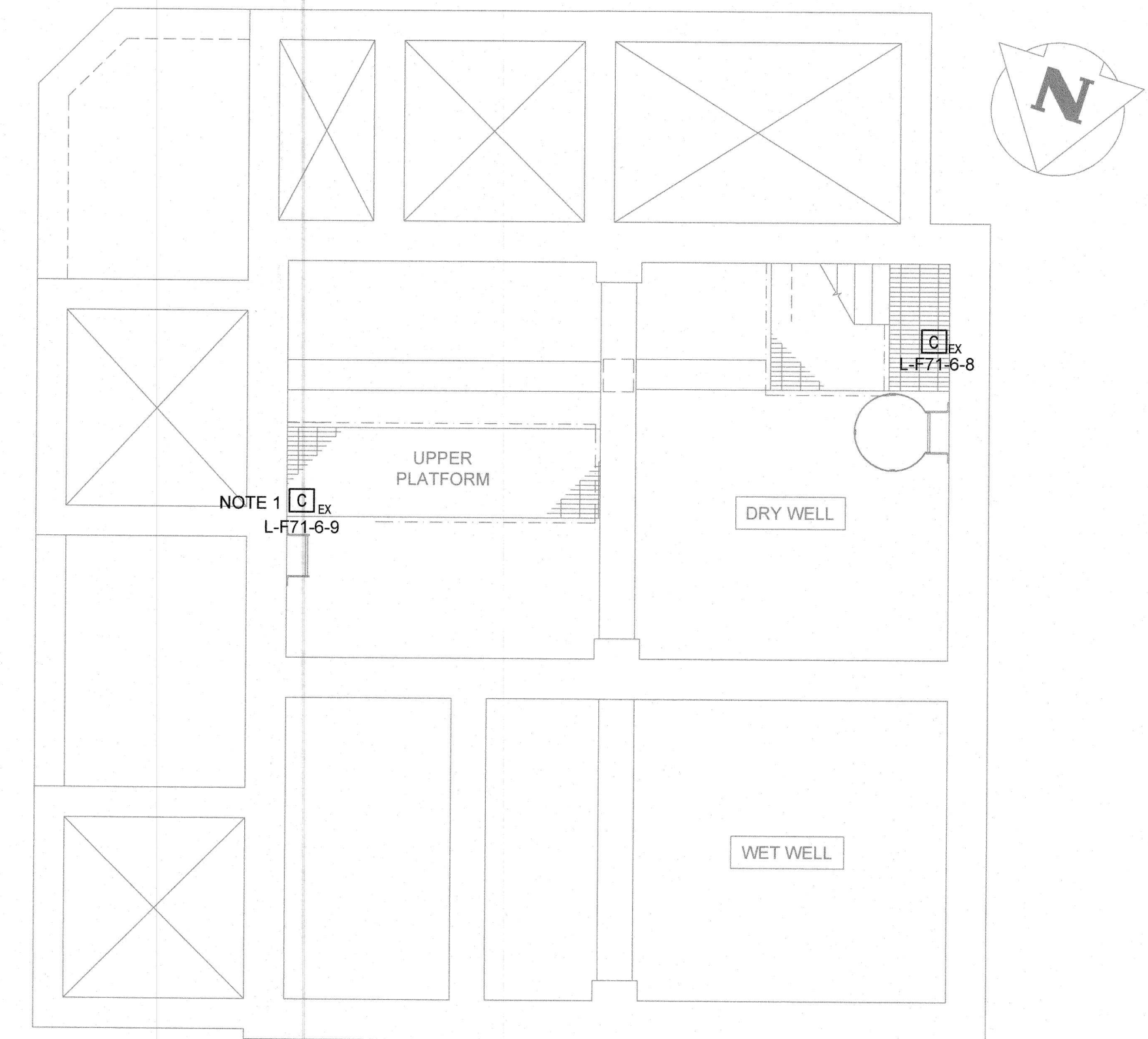
6 DRY/WET WELL PLAN 1:50 T.O. PUMP FLOOR @ EL. 227.498
