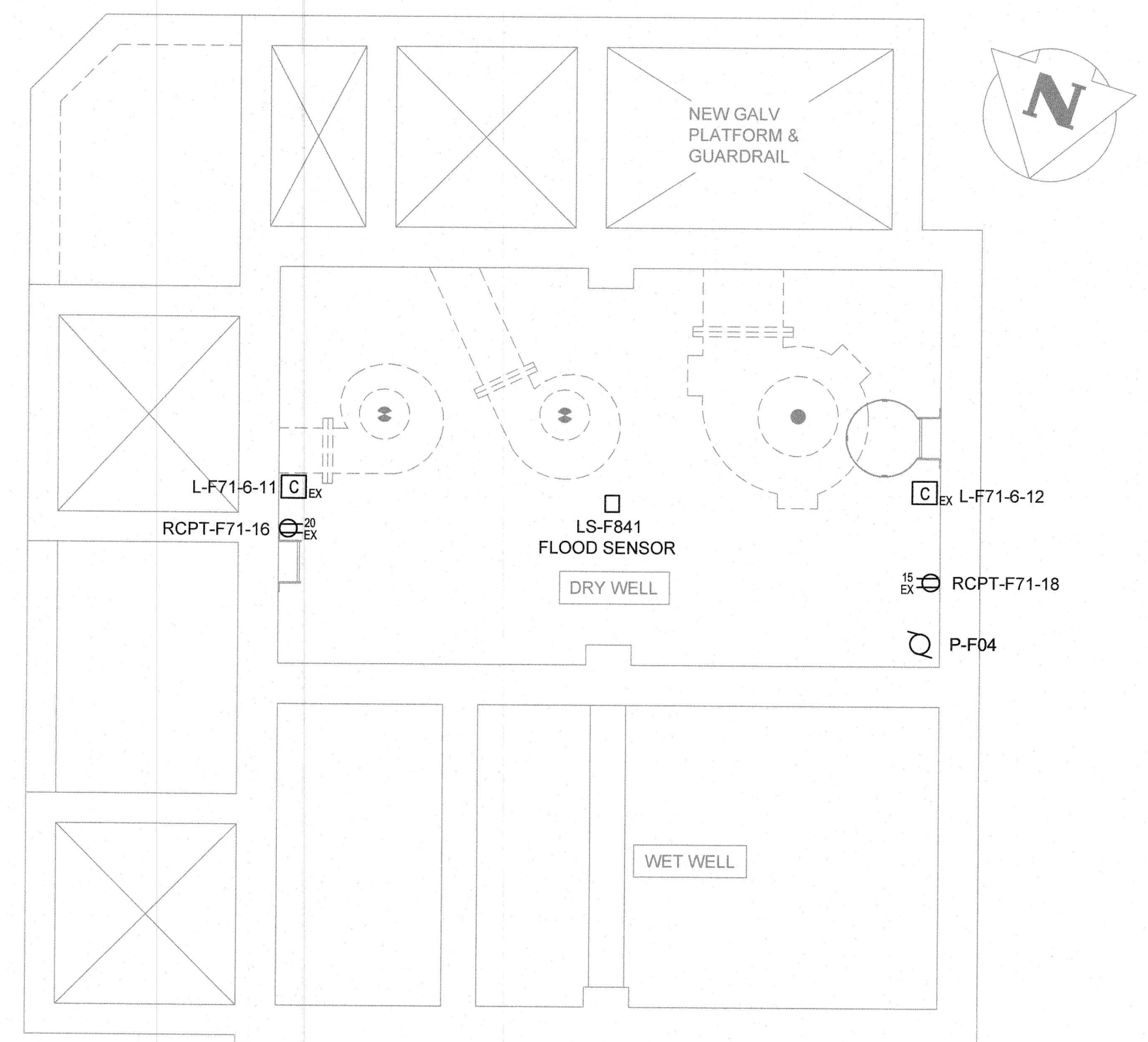
7 DRY/WET WELL PLAN 1:50 T.O. PUMP FLOOR @ EL. 221.914
