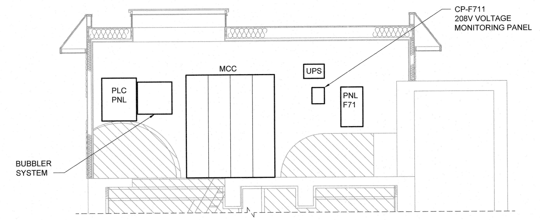
3 SECTION 1:50
