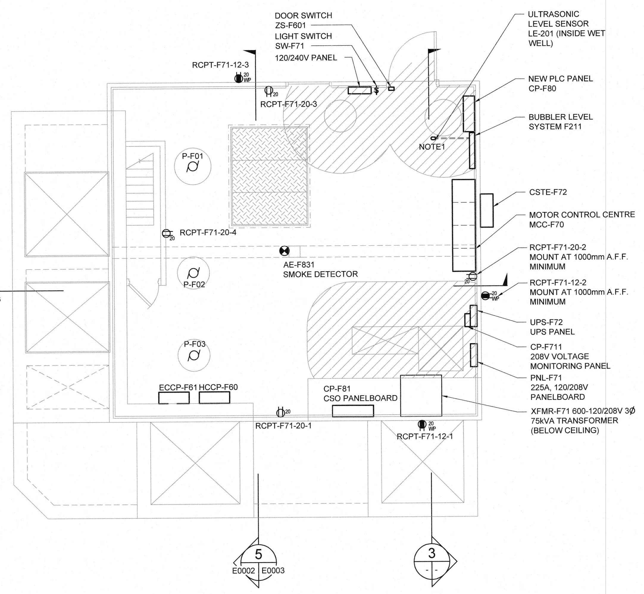
2 MAIN FLOOR PLAN - POWER 1:50
