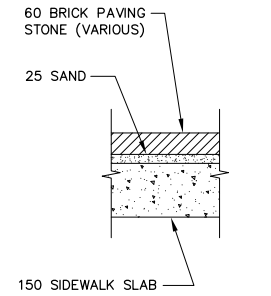
PAVING DETAIL (TYP) N.T.S.
