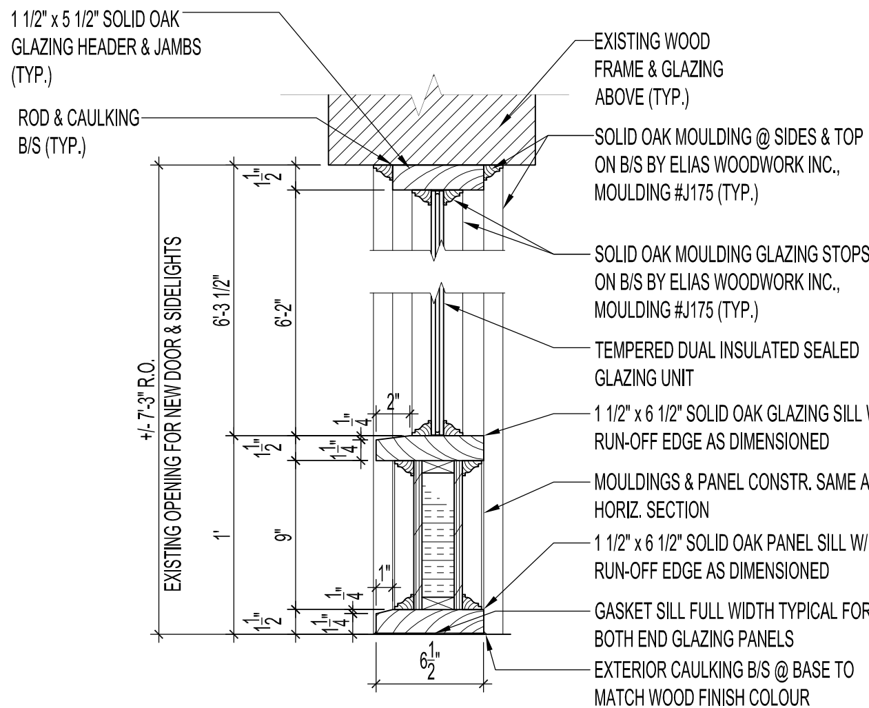
SECTION -EXTERIOR GLAZING & PANEL -DOOR D101A SCALE: 1 1/2" =1'-0"
