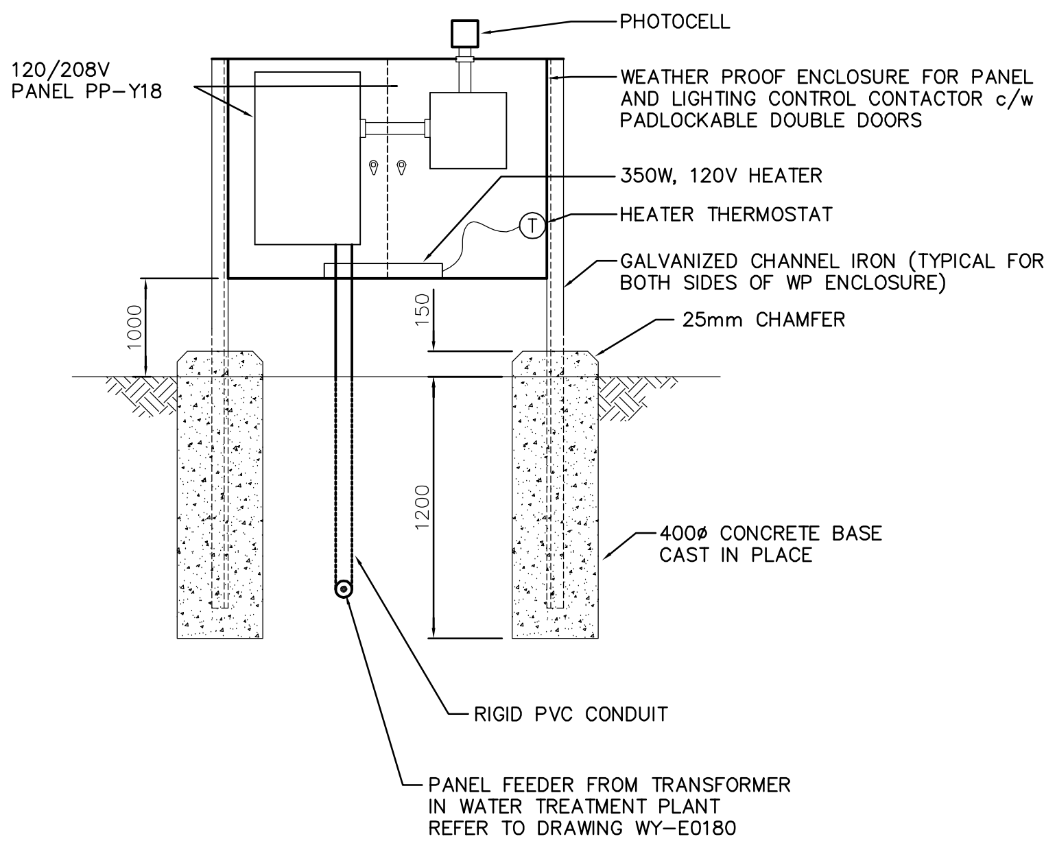
B PARKING PANEL PP-Y18 DETAIL WY-E0180 SCALE: NTS B WY-E0181
