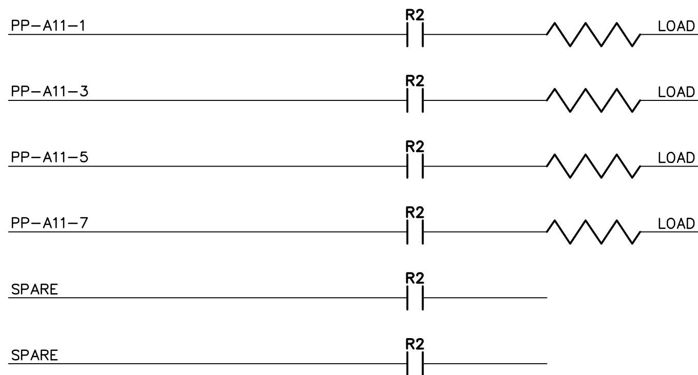
F ROADWAY LIGHTING CONTROL LCP-A11 DETAIL WY-E0481 SCALE: NTS
