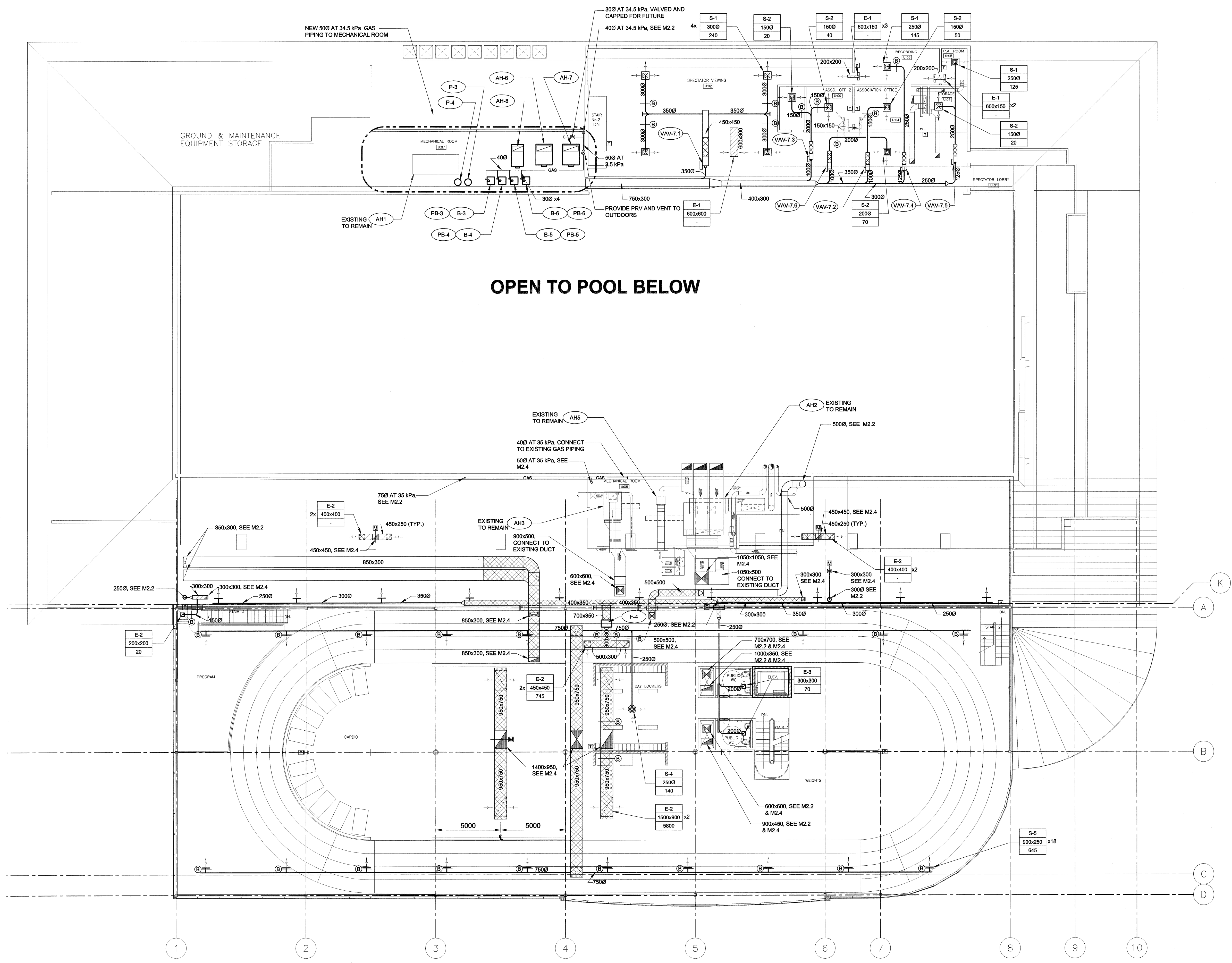
PLAN 1 M2.3 SCALE 1:150 SECOND FLOOR HVAC NEW CONSTRUCTION
